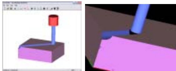
Fig. 6. Masim program
